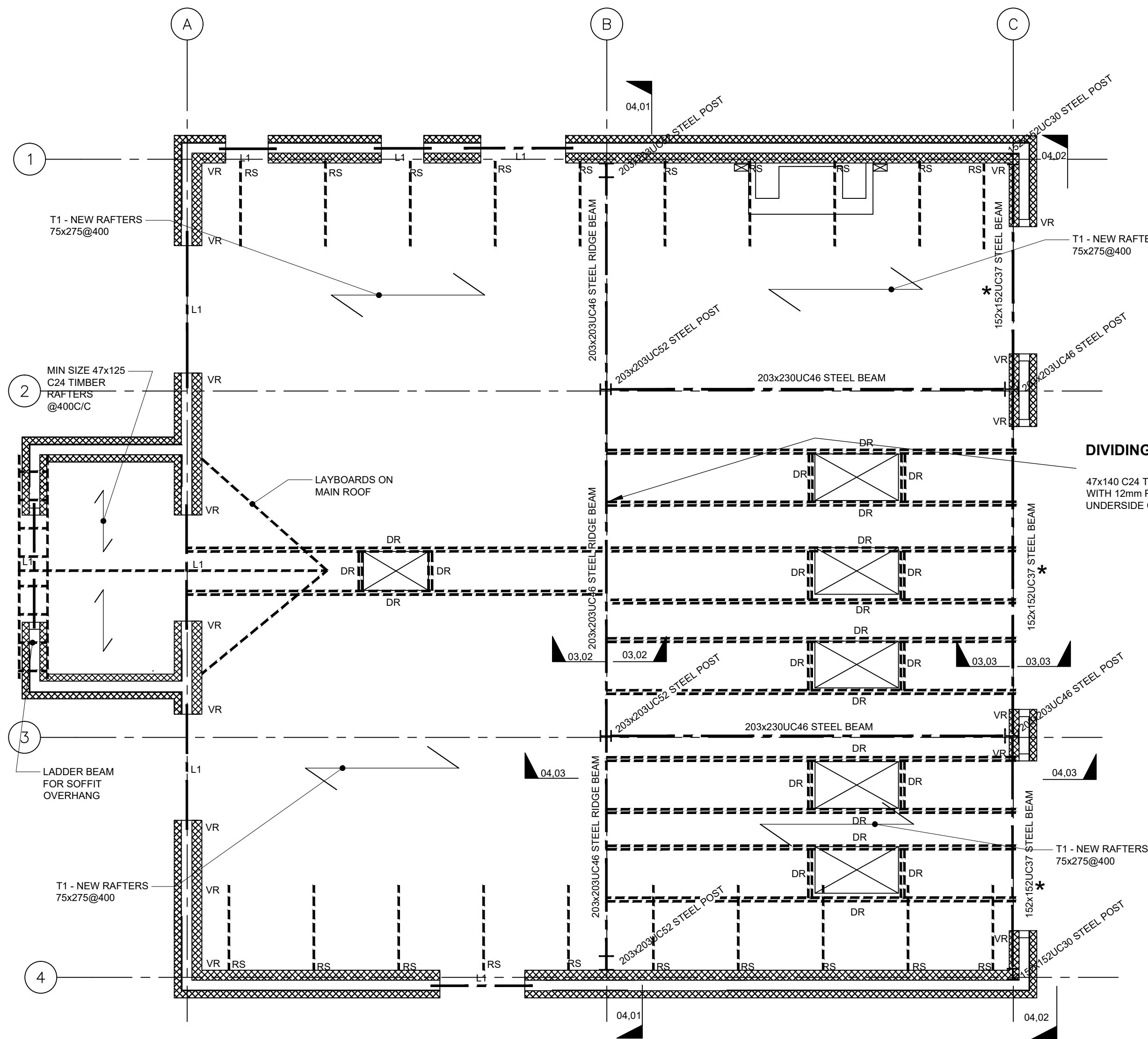
03,01 ROOF PLAN SHOWING NEW MEMBERS
