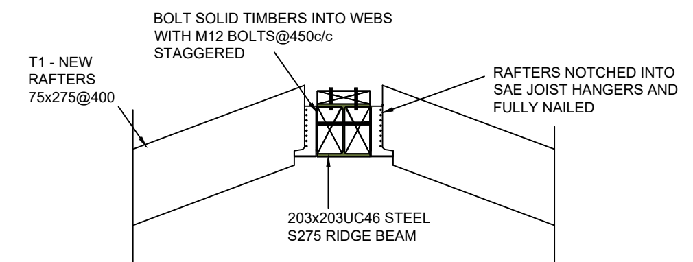
03,02 RIDGE DETAIL
